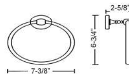
ITR2080 Norville, Towel Ring
