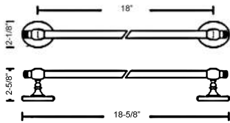
ITB2080- 18 Norville, 18" Towel Bar
