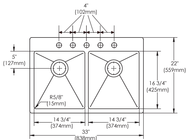
Model ECTSR33229BG5 Illustrated
