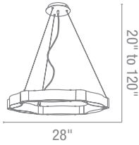
62317 Titanium Chandelier 6Lt x 100w Halogen 120v J78 (T-3 Base) Finish BS Glass FST Included 10ft of Cable & Cord CETL Dry
