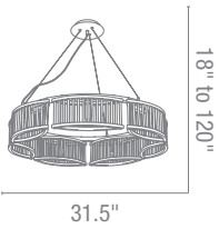
23979 Gemini Crystal Chandelier 7Lt x 75w Halogen 120v JCD (G-9 Base) Finish CH Glass CCL Included 10ft of Cable & Cord CETL Damp
