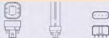
G24q-3 L-PLC26W/27 2G11 Base 26W G24q-3 Base Base
