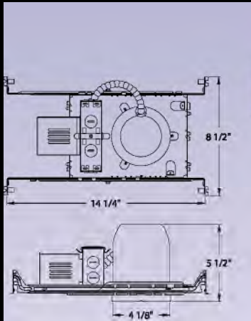
V8408 Non-IC, Non-Air Tight, 50W
