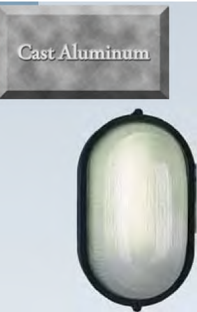
✦ V6880-5 Black Frosted Ribbed Glass 6½"W × 11"H × 5¼"E 1×13W GX23 120V NPF Magnetic
