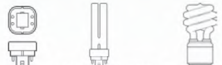
G24q-1 L-PLC13W/827 L-ESS13W Base 13W GU24 Base 13W GU24 Base
