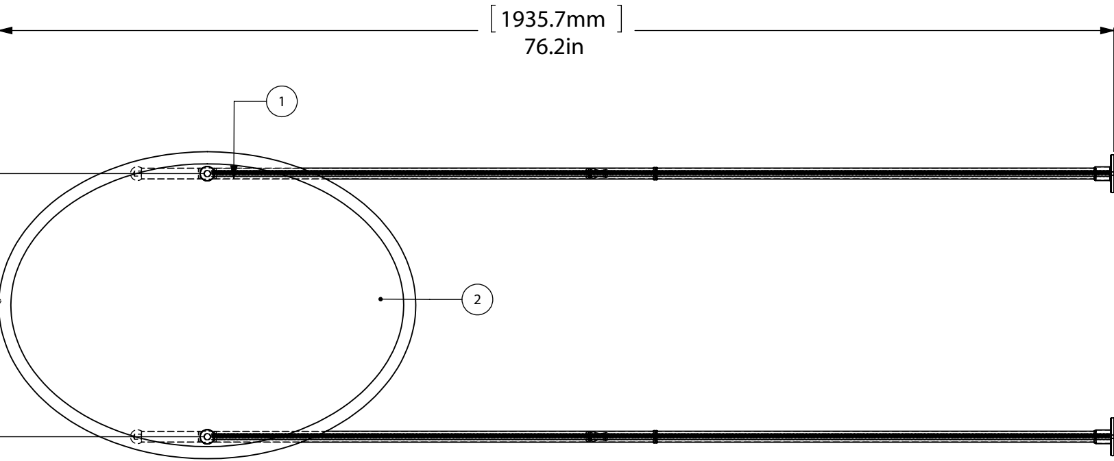
DETAIL L SCALE 1 : 3
