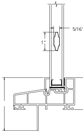
1" CONTOUR GBG BAR
