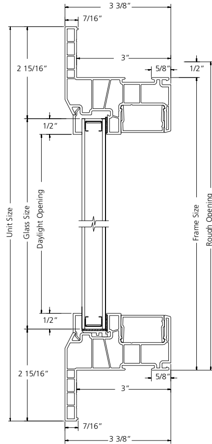
VERTICAL SECTION
