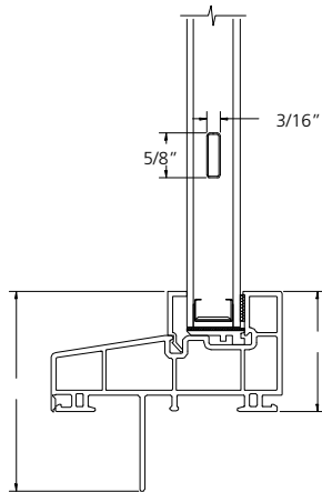
5/8" FLAT GBG BAR
