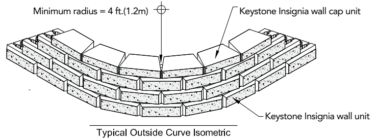
Typical Outside Curve Isometric
