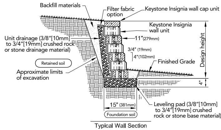
Typical Wall Section
