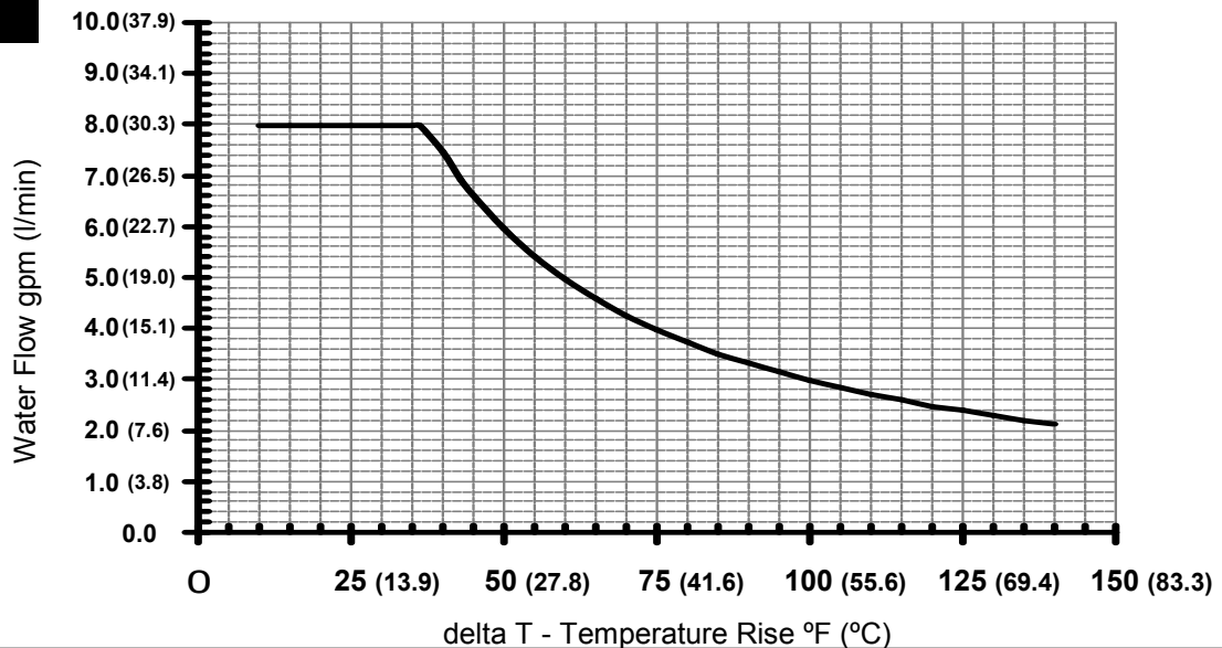
FLOW TABLE
