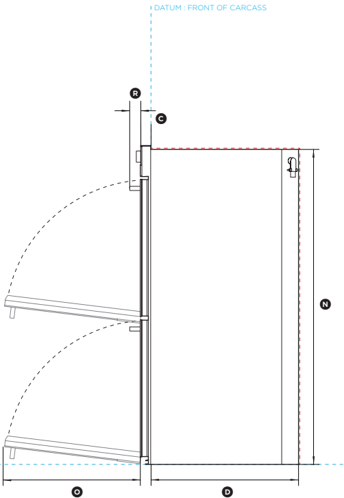
PROFILE VIEW
