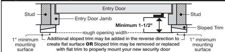
Figure 4 Stucco 1 - Surface Mount
