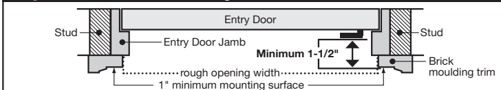
Figure 2 Flat Trim - Surface Mount
