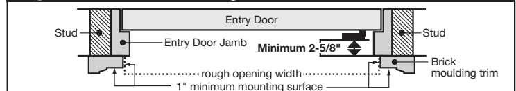
Figure 2 Flat Trim - Recessed Mount
