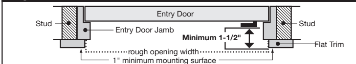
Figure 3 Sloped Trim - Surface Mount
