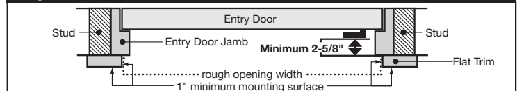
Figure 3 Sloped Trim - Recessed Mount
