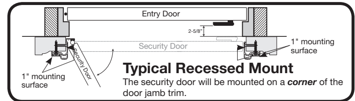
Figure 1 Brick Molding - Recessed Mount
