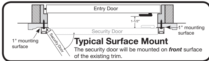
Figure 1 Brick Molding - Surface Mount
