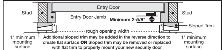
Figure 4 Stucco - Recessed Mount
