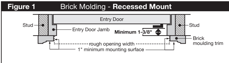
Typical Recessed Mount
