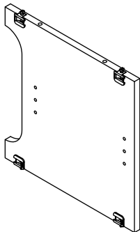
(7) MIDDLE DIVIDER (1 PC)
