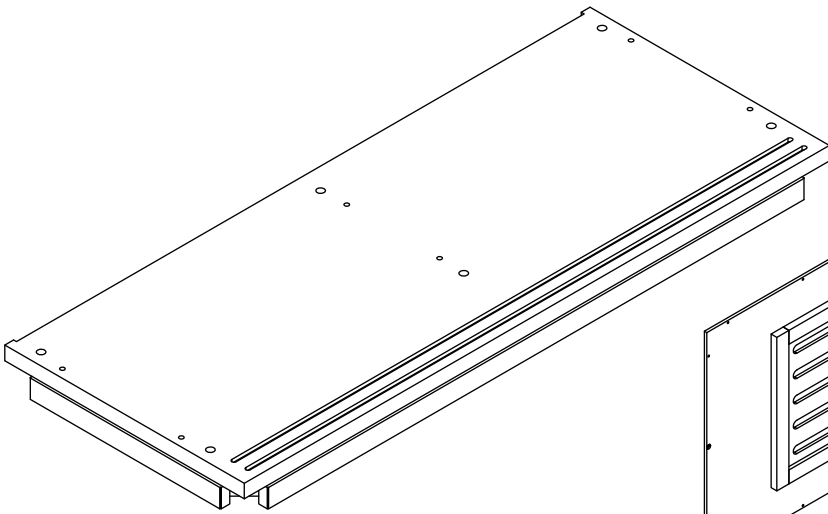
(3) BOTTOM PANEL (1 PC)
