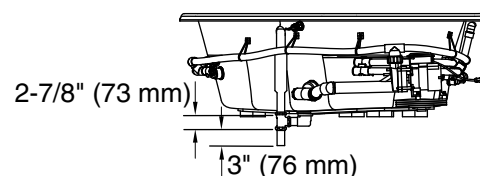
27-1/2" (699 mm) Drop-In Rim Style Cut-Out Detail
