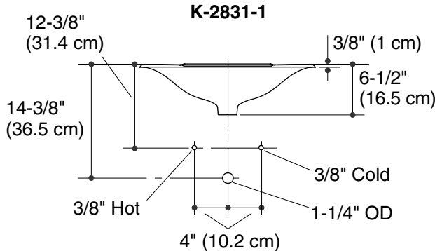
Standard Installation
