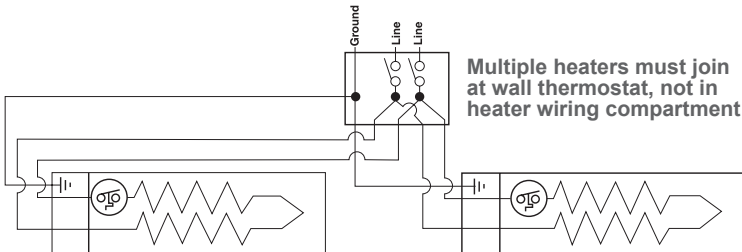
Connecting multiple units 240 or 208 volt models only Double pole wall thermostat left end wiring
