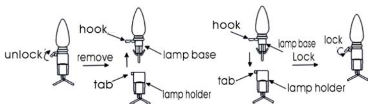
Fig.1 Unlock and remove the burned out lamp
