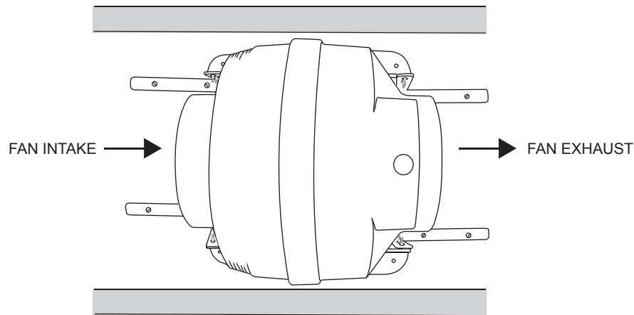
FIGURE 2: MOUNTING
