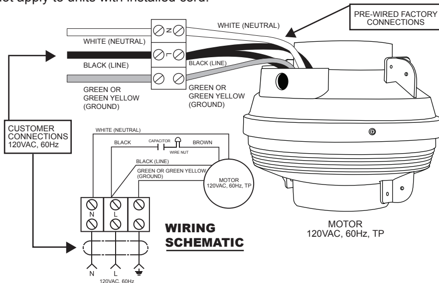
FIGURE 3: WIRING DIAGRAM
