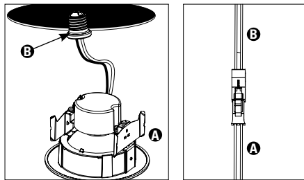
Figure 5. Retrofit Connection
