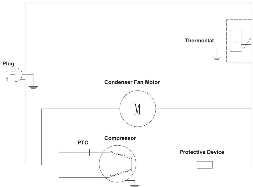
Electric Wiring Diagram
