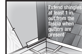
Figure 14 Valley/Shingle Extension
