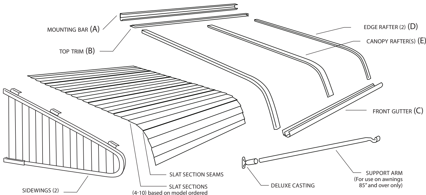
Series 1500 with Sidewings
