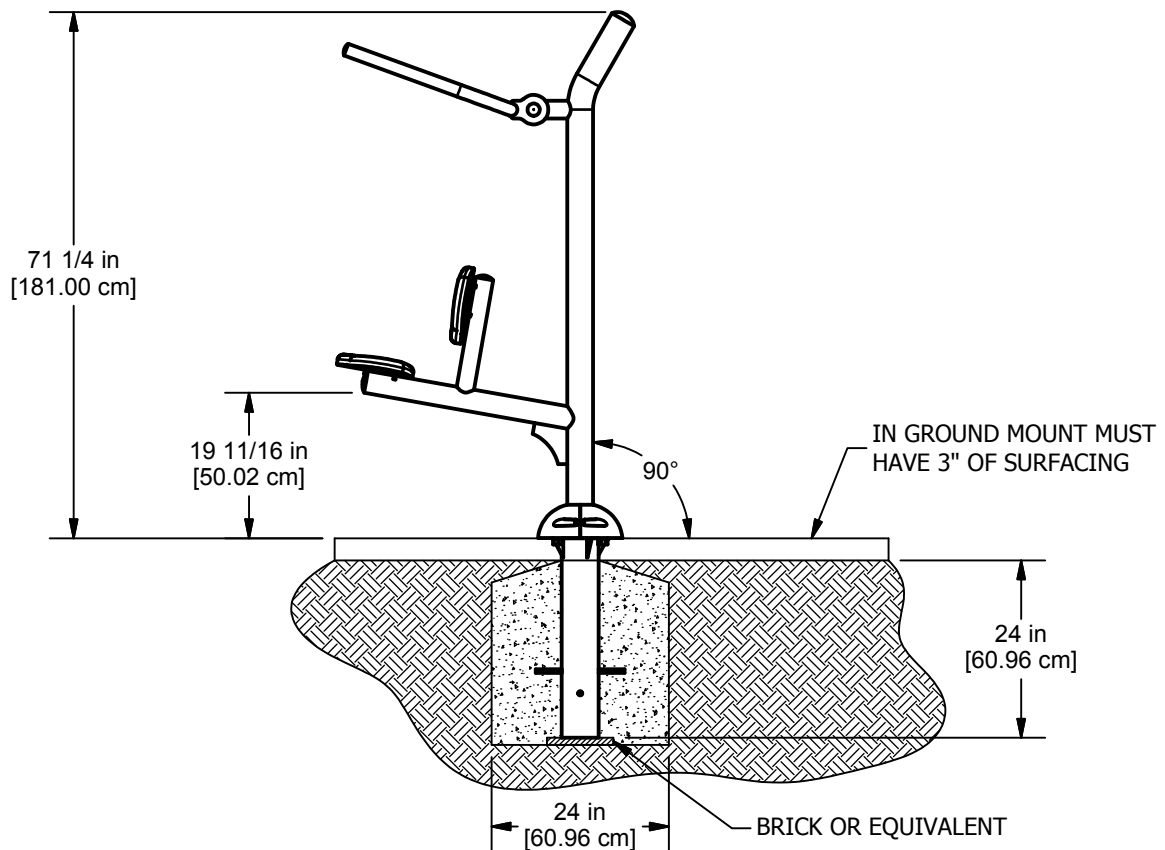
ELEVATION VIEW
