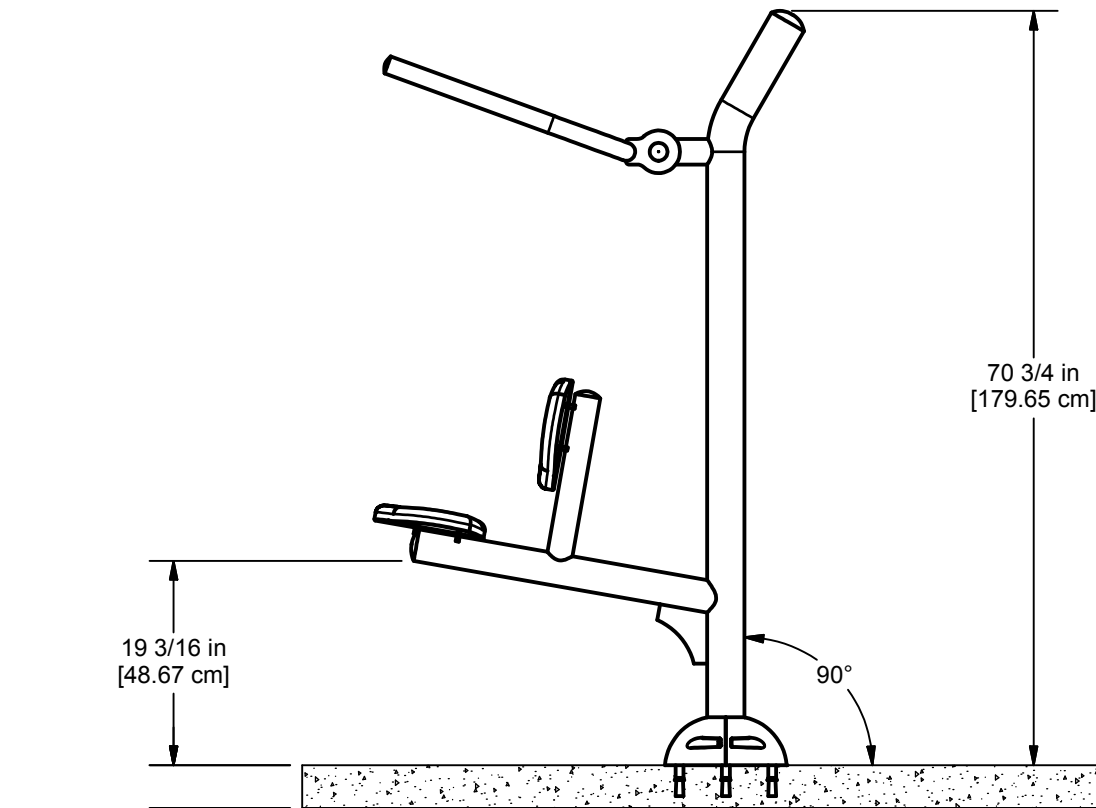
ELEVATION VIEW UP165S (SURFACE)
