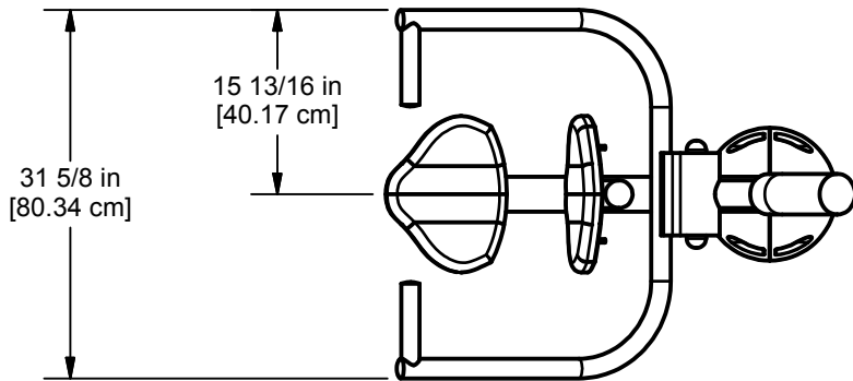
PLAN VIEW UP165S (SURFACE)
