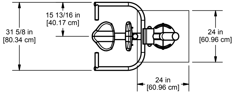
PLAN VIEW
