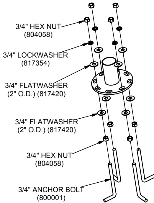
FOOTING ASSEMBLY DETAIL UP165F (FOOTING)
