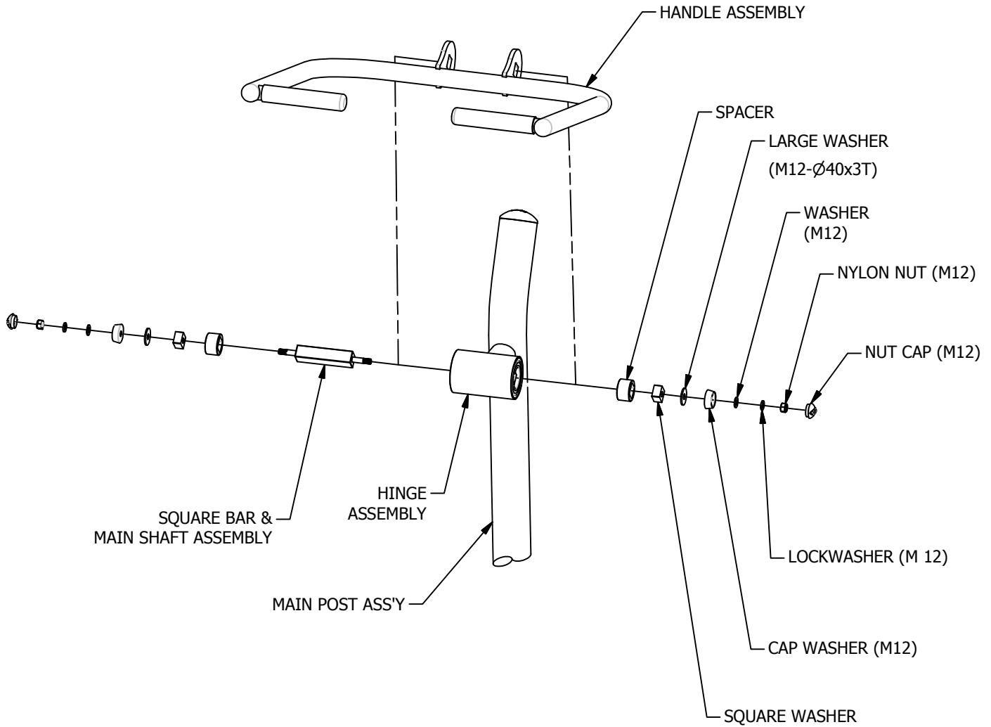
HANDLE ASSEMBLY DETAIL
