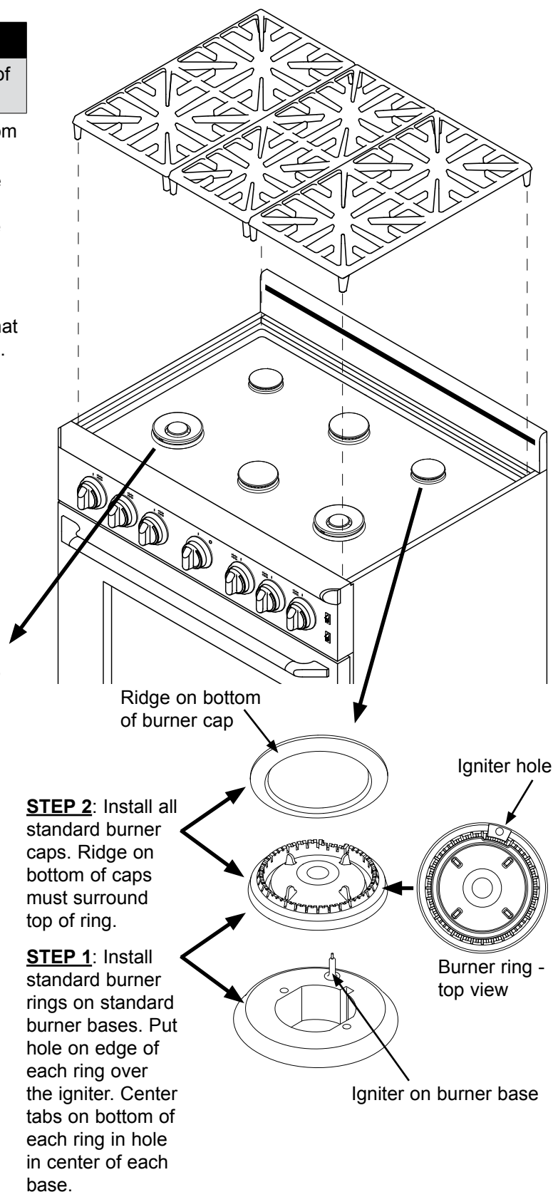
Standard Burner Assembly (left rear, right rear and both center burners)
