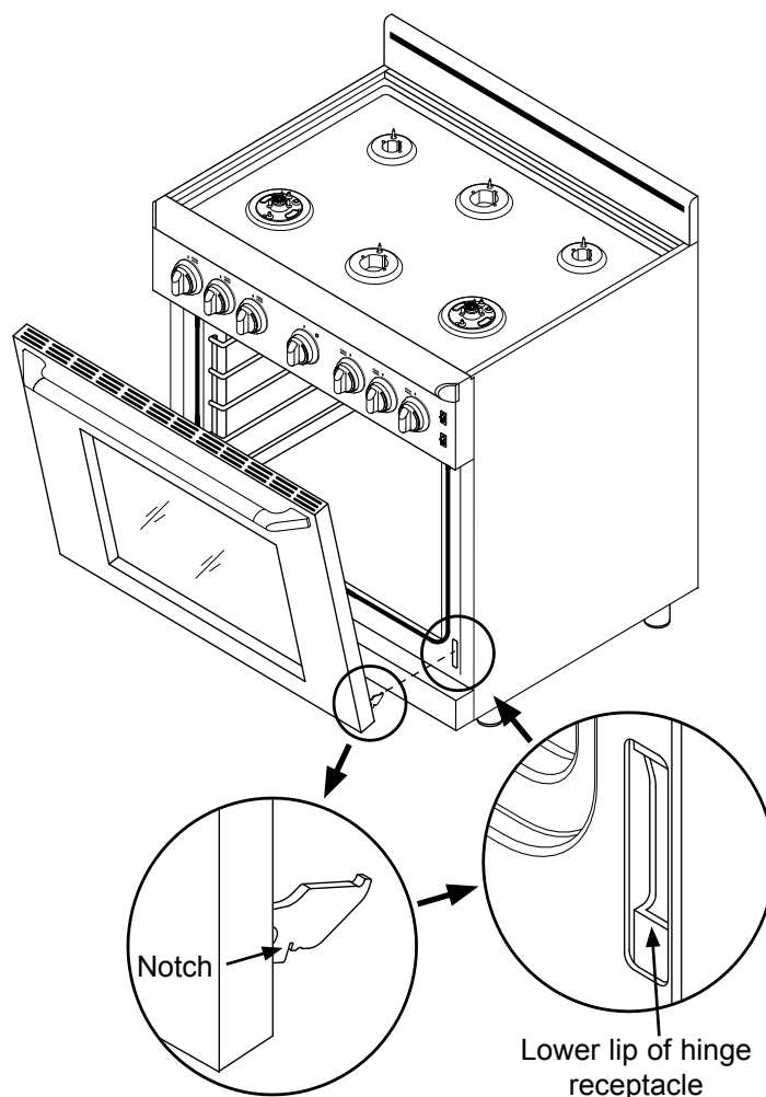
Door Installation
