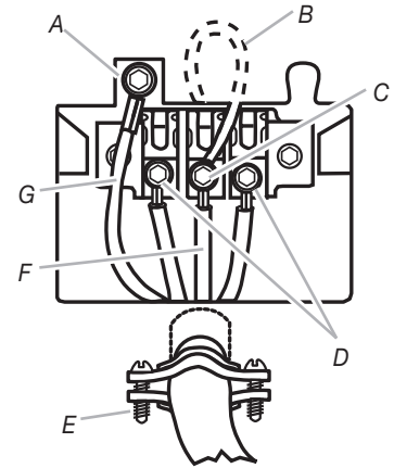
A. External ground conductor screw B. Appliance neutral ground wire C. Center terminal block screw D. Outer terminal block screws E. Strain relief screw F. Neutral (center wire) G. Ground wire
