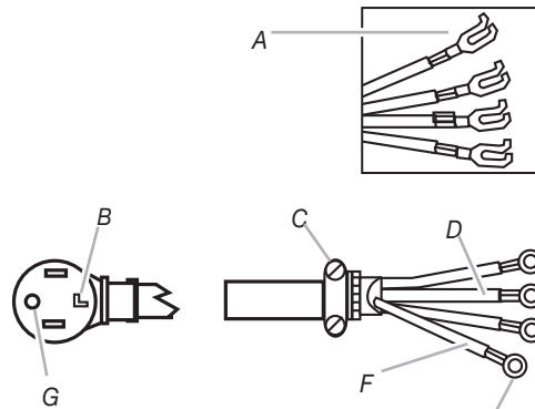
A. Spade terminals with upturned ends B. Neutral C. 3/4" UL-listed strain relief D. Neutral (white) E. Ring terminals F. Ground wire G. Ground prong
