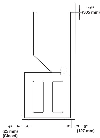
Front/Back/Top Clearances
