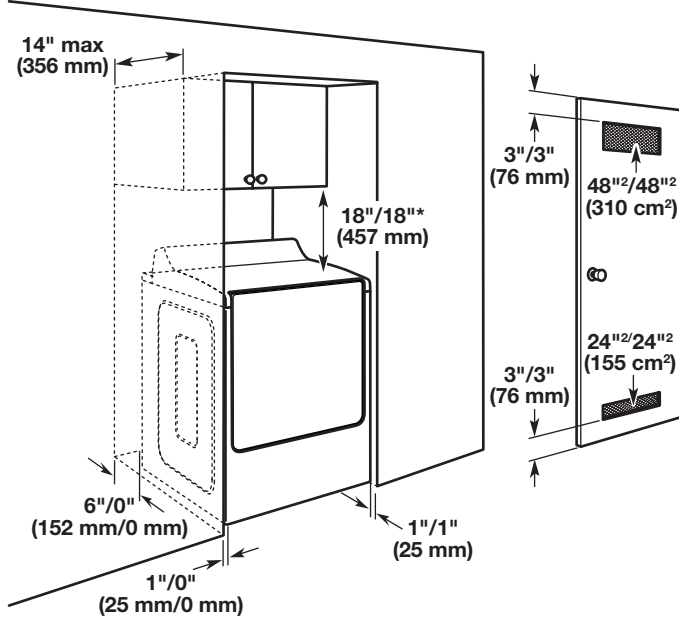
Recommended/Minimum spacing
