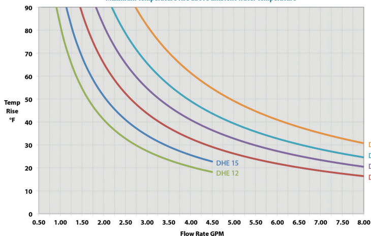
Temperature Rise versus Flow Rate @ 240 V
