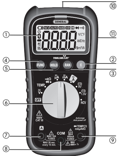
Fig. 1. The DMM's controls, indicators and physical features
