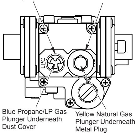
Figure 10 - Gas Regulator
