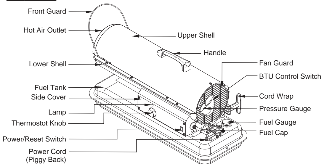
Figure 1. KFA80C MODEL
