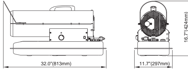
KFA80C Model
