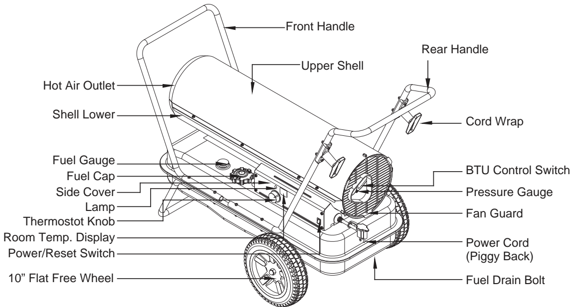
Figure 2. KFA135C MODEL
