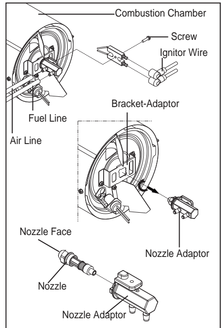
Figure 14. Nozzle Replacement
