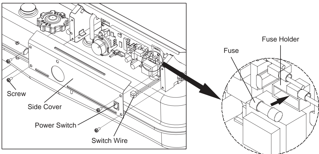
Figure 21. Replacing Fuse
