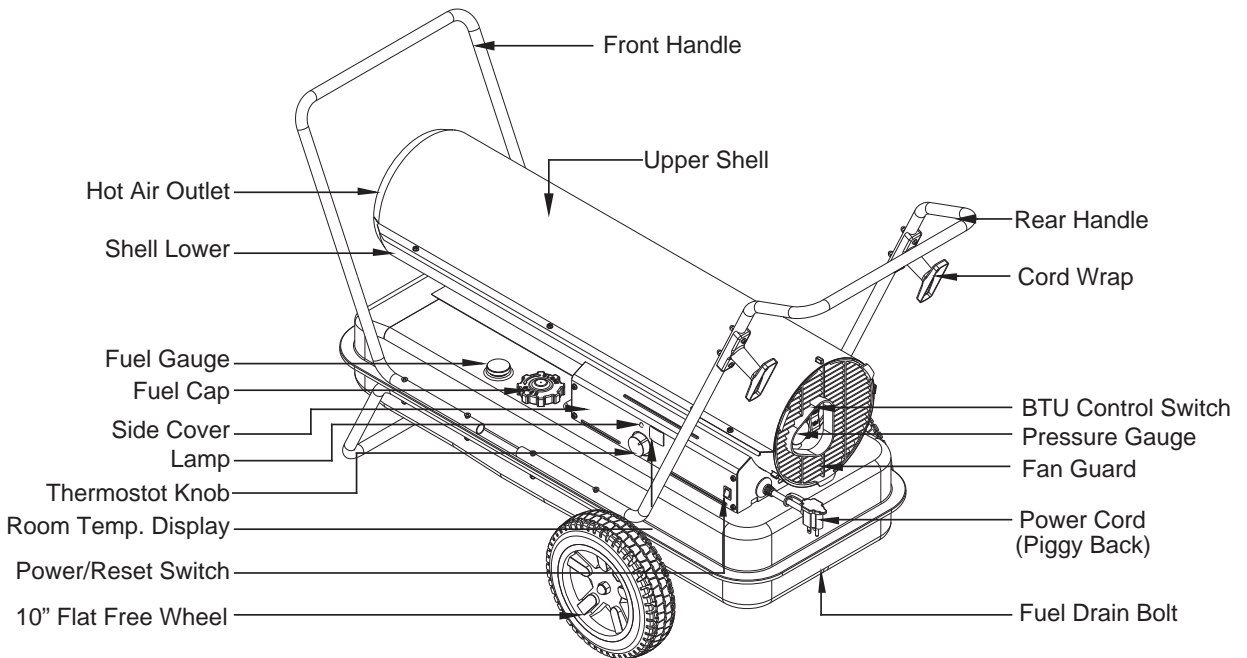
Figure 3. KFA220C MODEL
