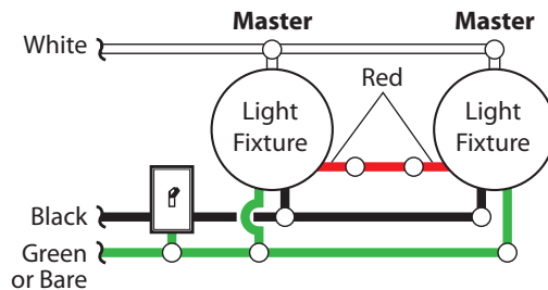
Wiring Diagram 3
