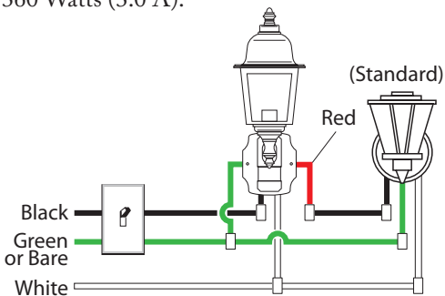
Wiring Diagram 1
