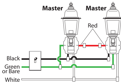
Wiring Diagram 3
