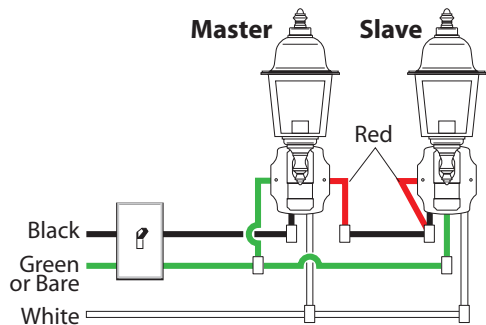
Wiring Diagram 2
