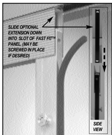
FIG. 3 - PANEL BUMPER SEAL
