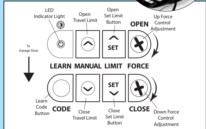
FIG. 6-1 Limit controls.
