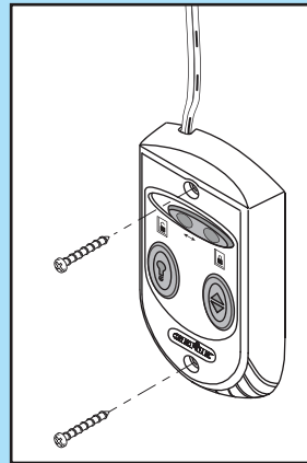
FIG. 3-4 Mounting Wall Console.
