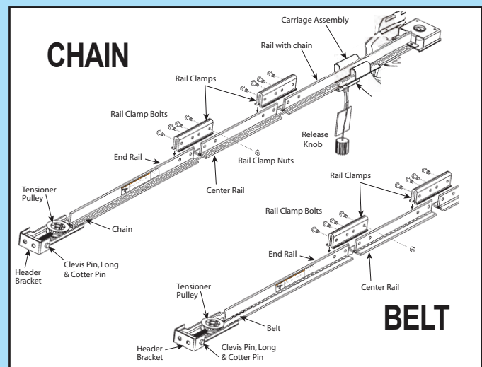
FIG. 1-2 Split Rail sections.
