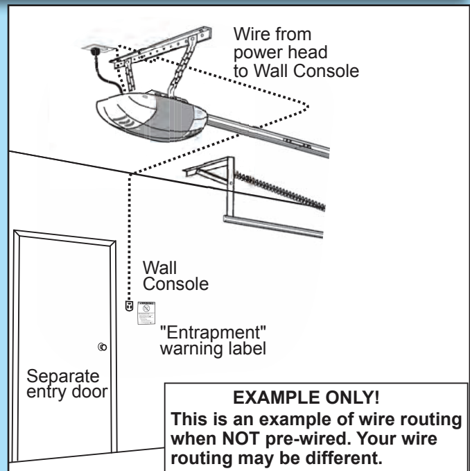
FIG. 3-1 Wall Console wire routing
