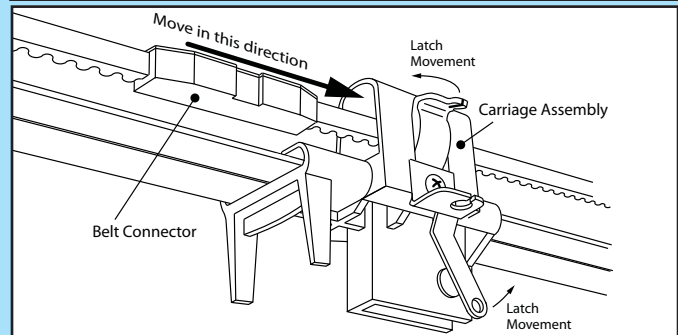
FIG. 6-2 Engage Chain/Belt Connector to Carriage.
