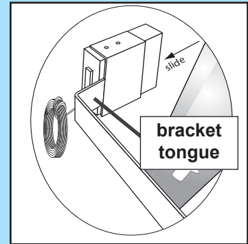
FIG. 4-3 Attach Safe-T-Beam® to brackets
