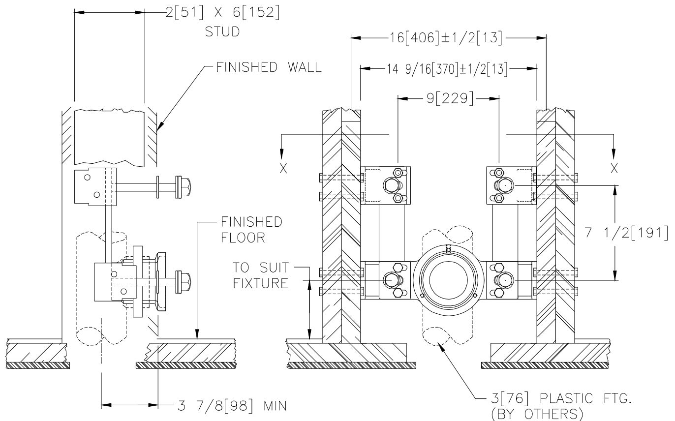
SECTION X-X
