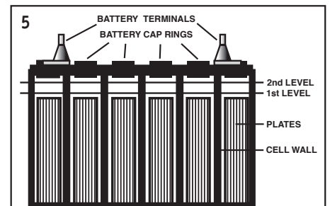
CROSS SECTION OF BATTERY 1. FILL TO 1st LEVEL, COVER THE PLATES 2. THEN FILL TO 2nd LEVEL, JUST BELOW THE BOTTOM OF THE CAP RINGS
