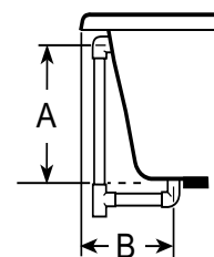
DRAIN/OVERFLOW
