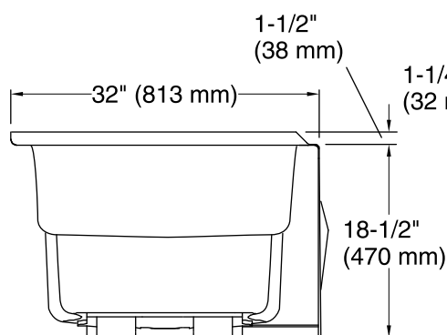
Integral Flange Detail
