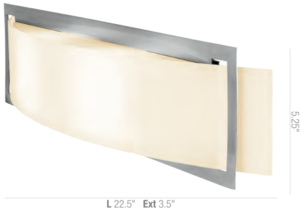
62105 Argon Wall Fixture 2Lt x 100w Halogen 120v J78 (T-3 Base) Finish BS Glass OPL CETL Damp Fluorescent Available ADA
