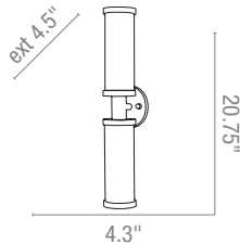
Vertical or horizontal mounting
