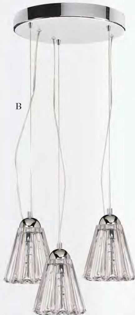
B. DHC593-12R-PC THREE LIGHT CRYSTAL PENDANT Polished Chrome Optical K9 crystal Canopy Dia: 12" (12cm) Glass: H: 6" (15cm) x Dia: 6" (15cm) Bulb: 9 x max. 20W G4 (not included)
