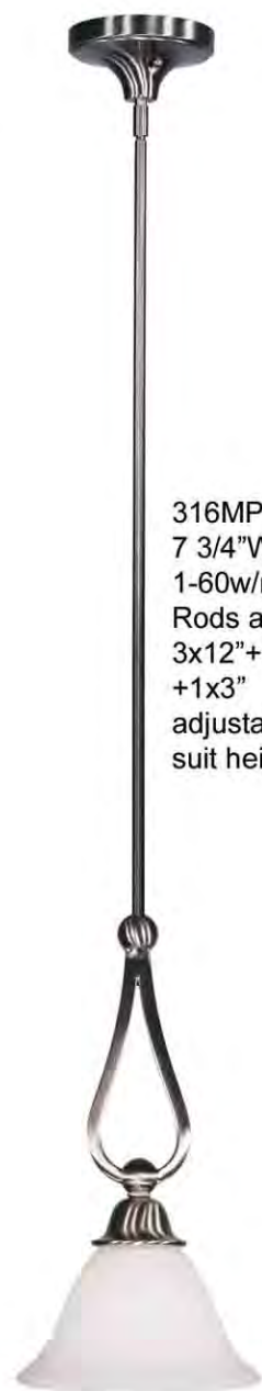
316P-14 14"W x 66 1/4"H 1-60w/m Rods are: 3x12"+1x6" +1x3" adjustable to suit height
