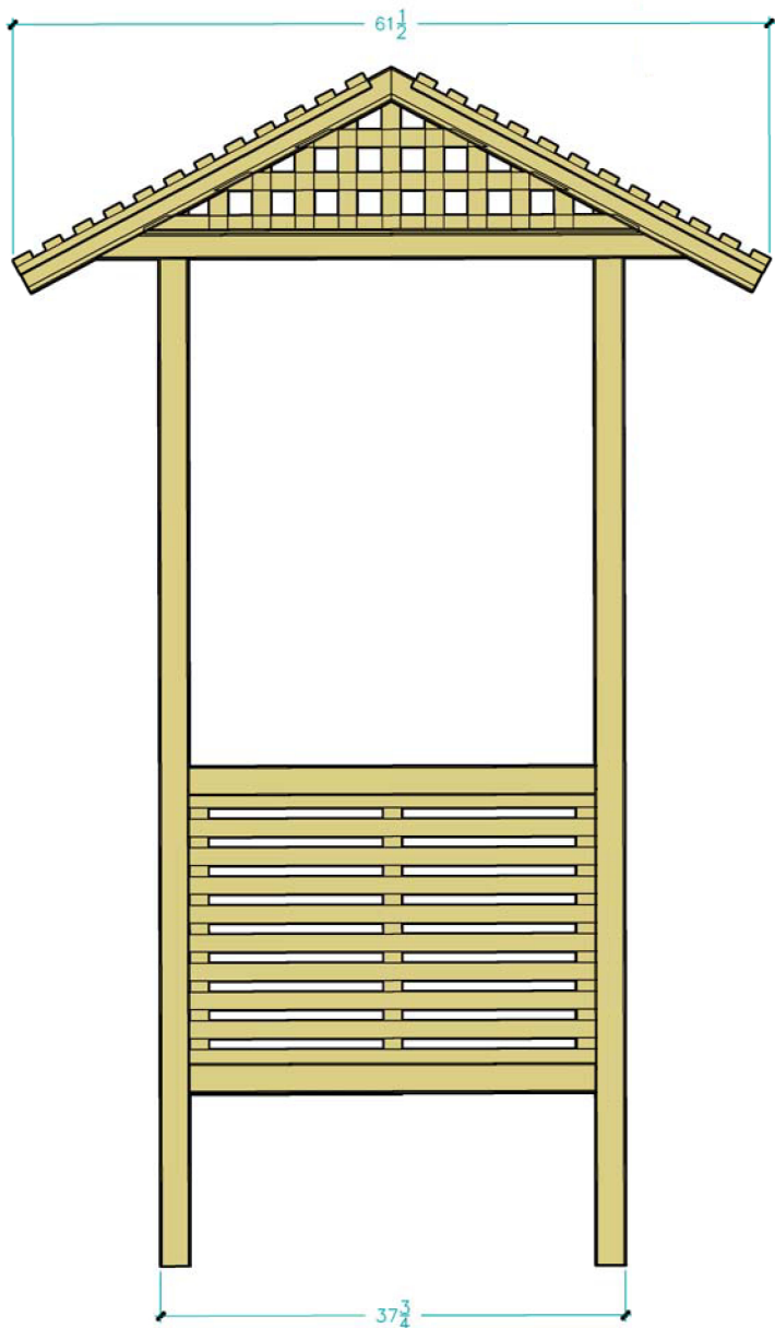
SIDE ELEVATION
