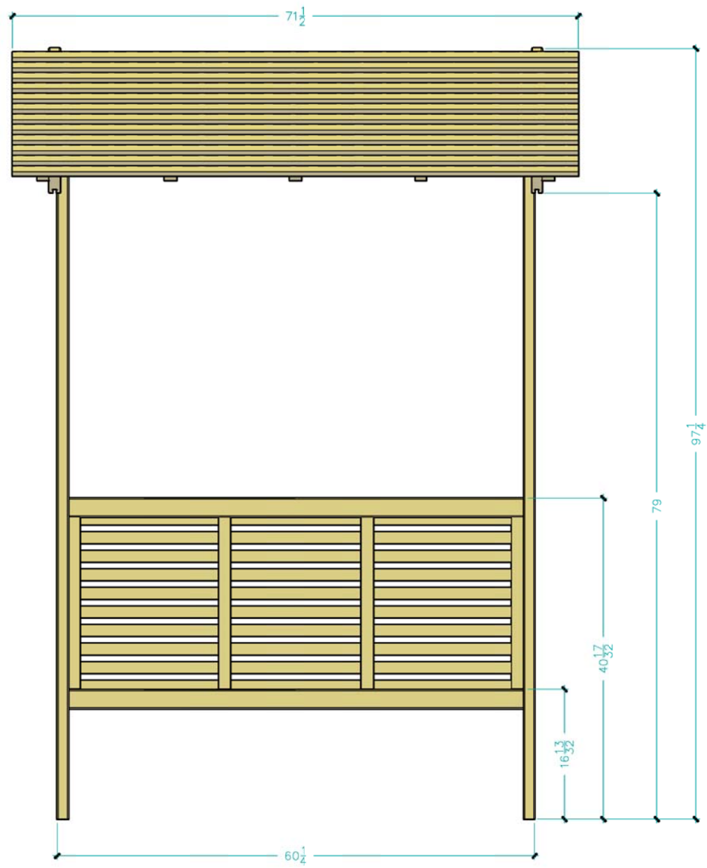
FRONT ELEVATION
