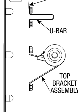
U-BAR PLACEMENT FOR TOP SECTION
