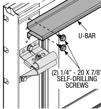
U-BAR PLACEMENT FOR TOP SECTION
