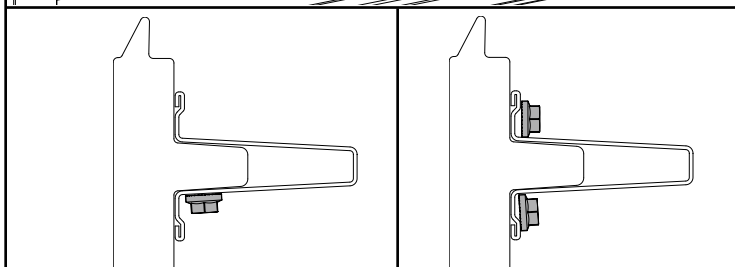
ATTACHING CENTER OF U-BAR
