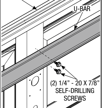
ATTACHING CENTER STILE
