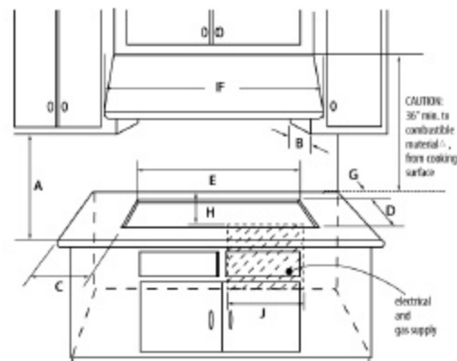
drop-in cooktop cut-out dimensions
