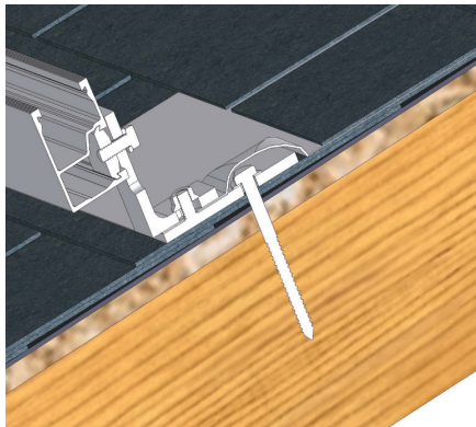
The Flashed L-Foot for composition roof attachment.
