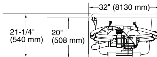
Integral Flange Detail
