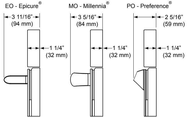
HANDLE DIMENSIONS - SIDE VIEW
