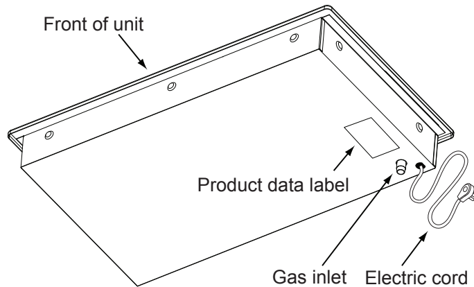
CHASSIS BOTTOM DIAGRAM
